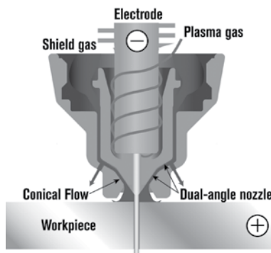
Conical Flow
